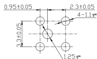
MOUNTING HOLE DIMENSIONS
