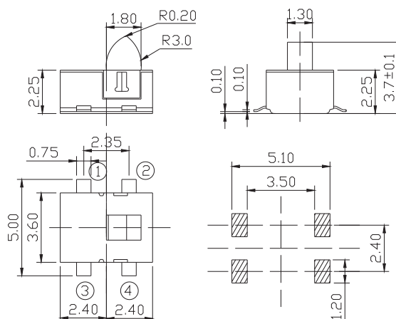
Pad layout
