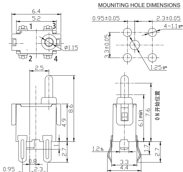
MOUNTING HOLE DIMENSIONS
